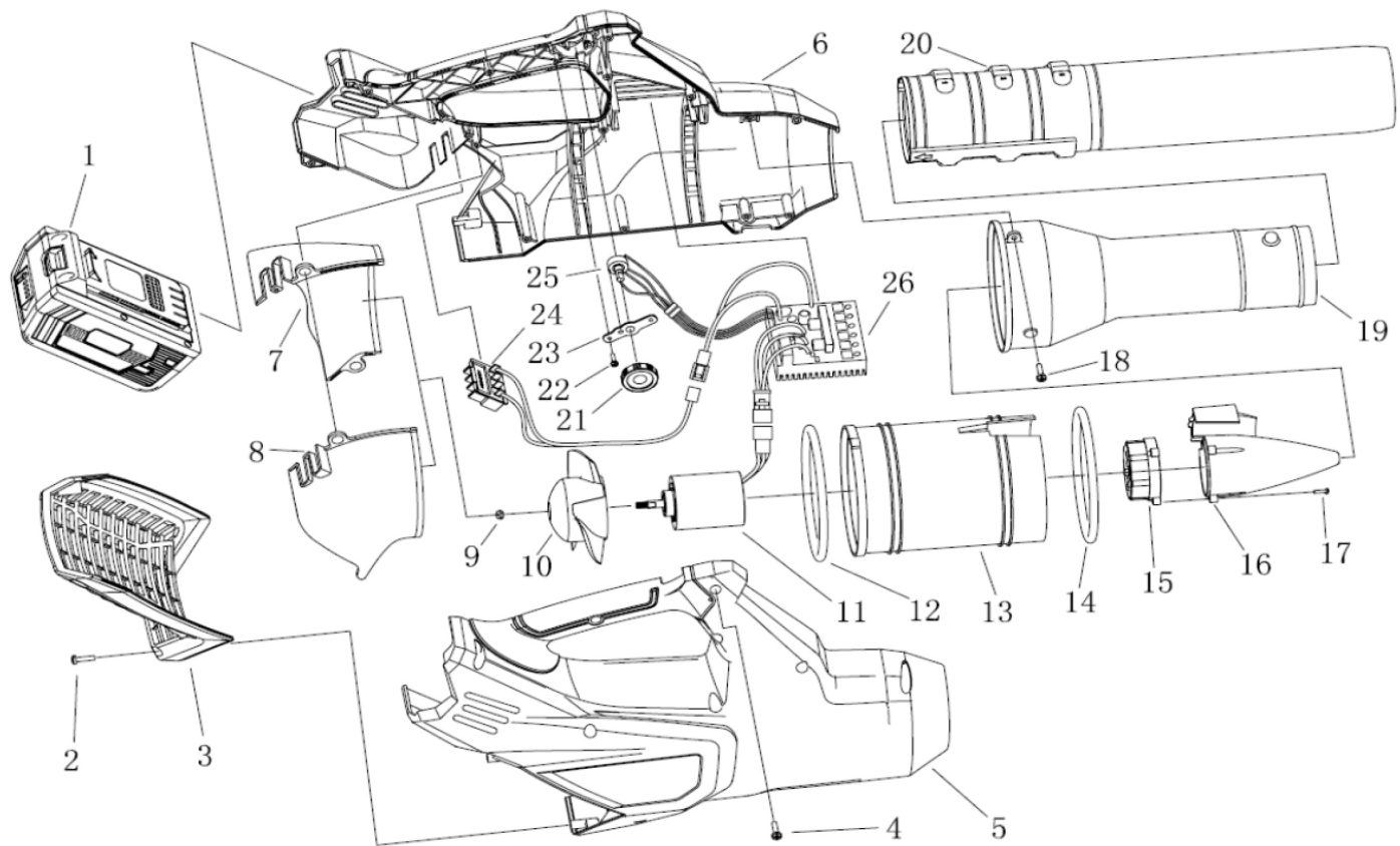
FIGURE 1 EXPLODED VIEW OF EB-36D
