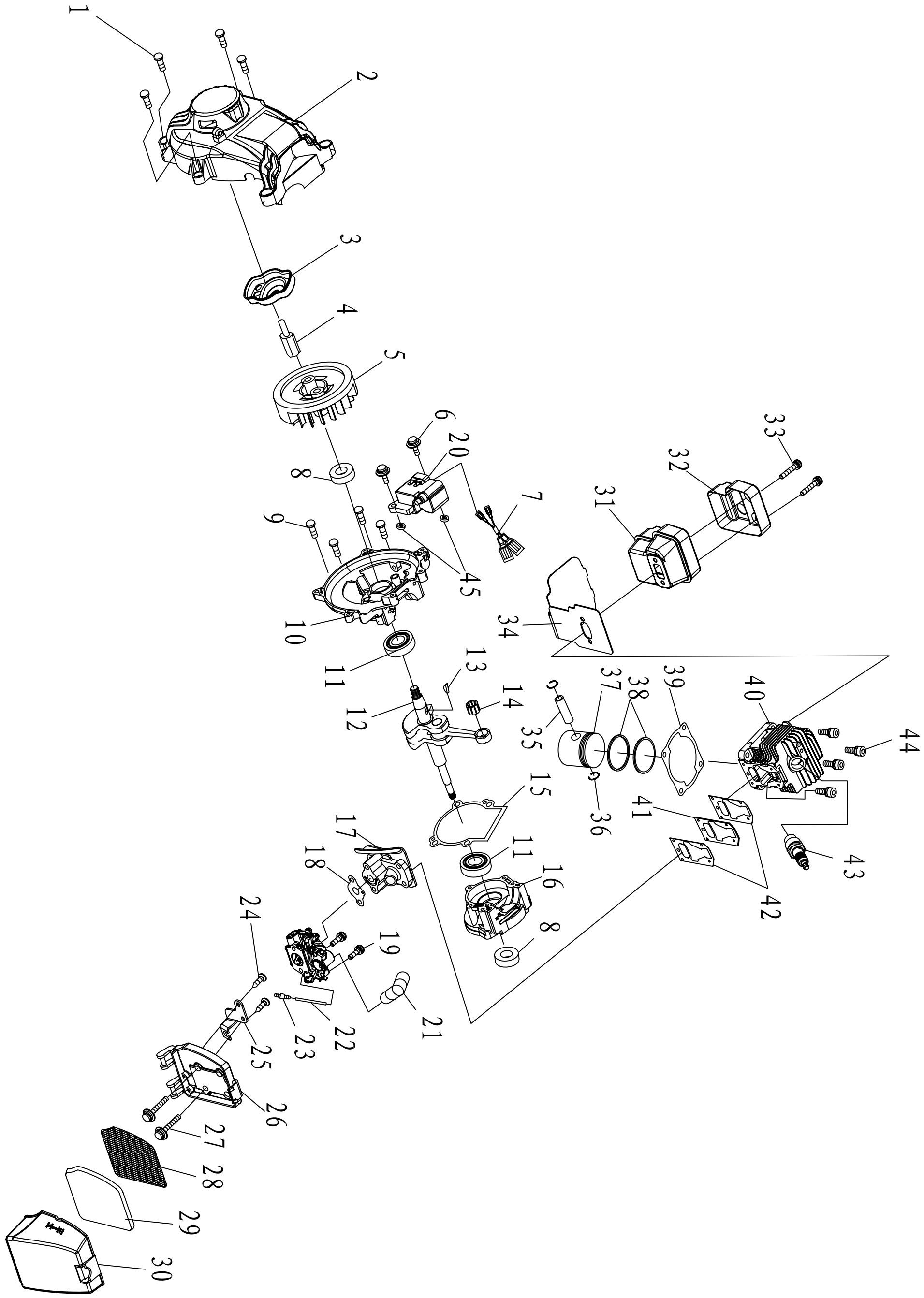
FIGURE 1 EXPLODED VIEW OF EBV260-3E.1
