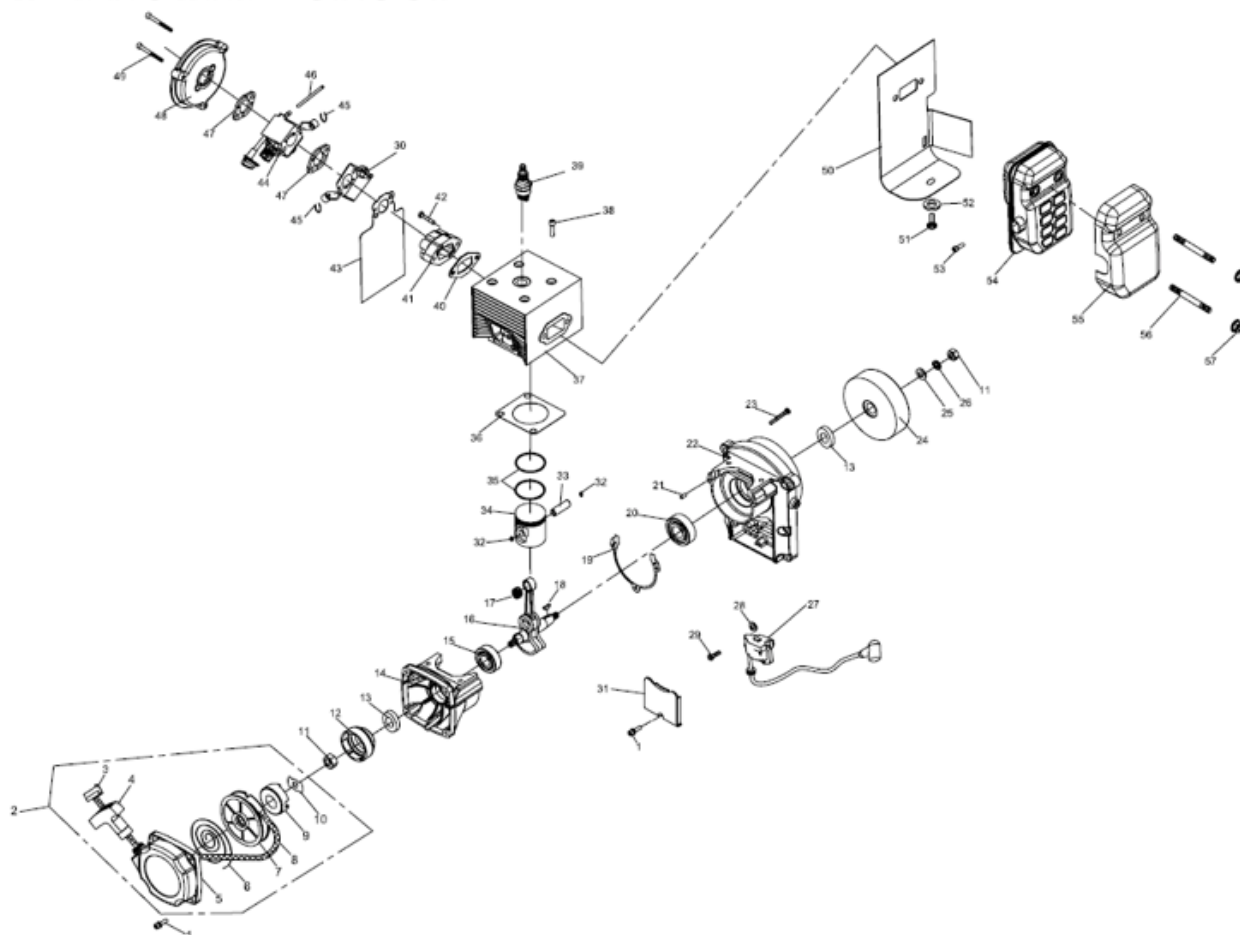
Fig. 1 ENGINE GROUP
